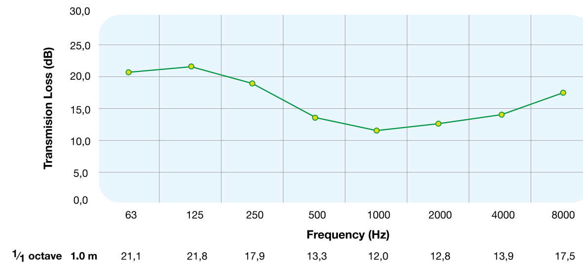
SOUNDROP AFS-NW - Ø 127 mm - 1.0 m
