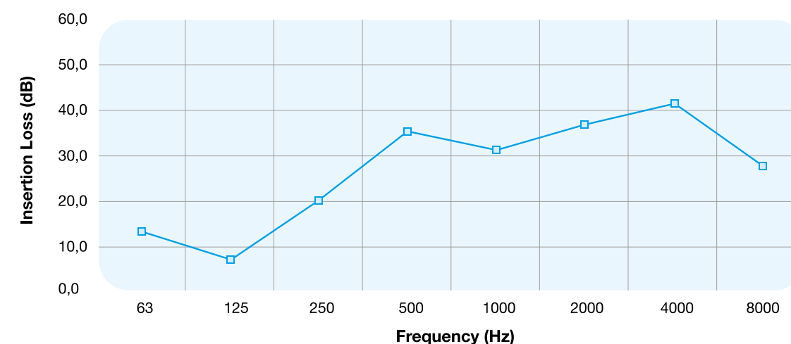
SOUNDROPAFS-NW - Ø 127 mm - 1.0 m
