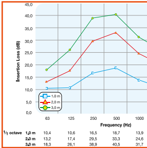
INSERTION LOSS DIAGRAMS
