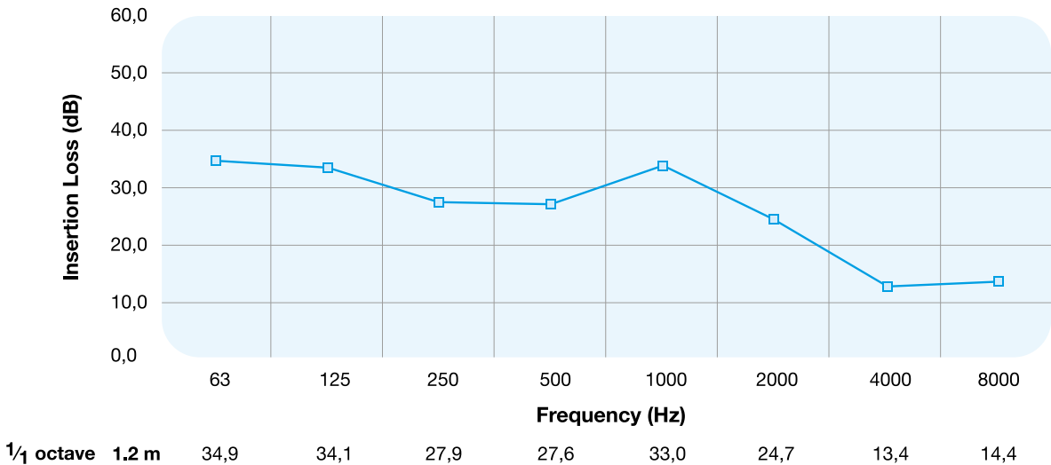
SOUNDROPAFS.P - Ø 160 mm - 1.2 m (50 mm Insulation)
