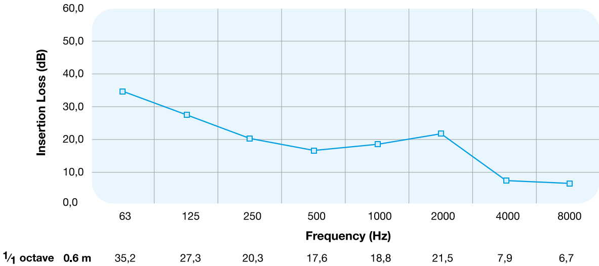
SOUNDROPAFS.P - Ø 160 mm - 0.6 m
