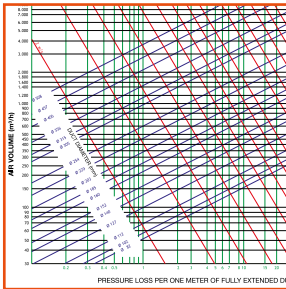
PRESURE LOSS DIAGRAMS
