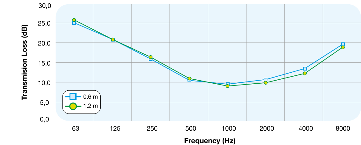
SOUNDROPAFS.P - Ø 100 mm
