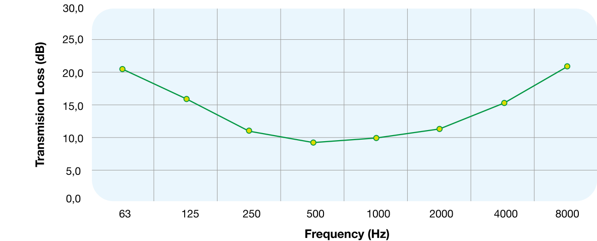
SOUNDROPAFS.P - Ø 160 mm - 1.2 m (50 mm Insulation)
